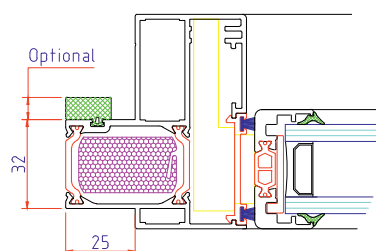
Detail B (2:1)
