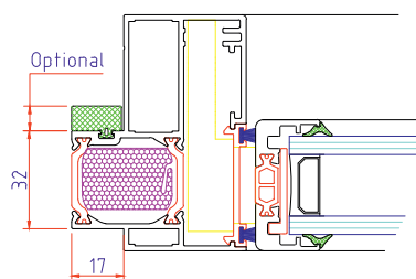
Detail A (2:1)
